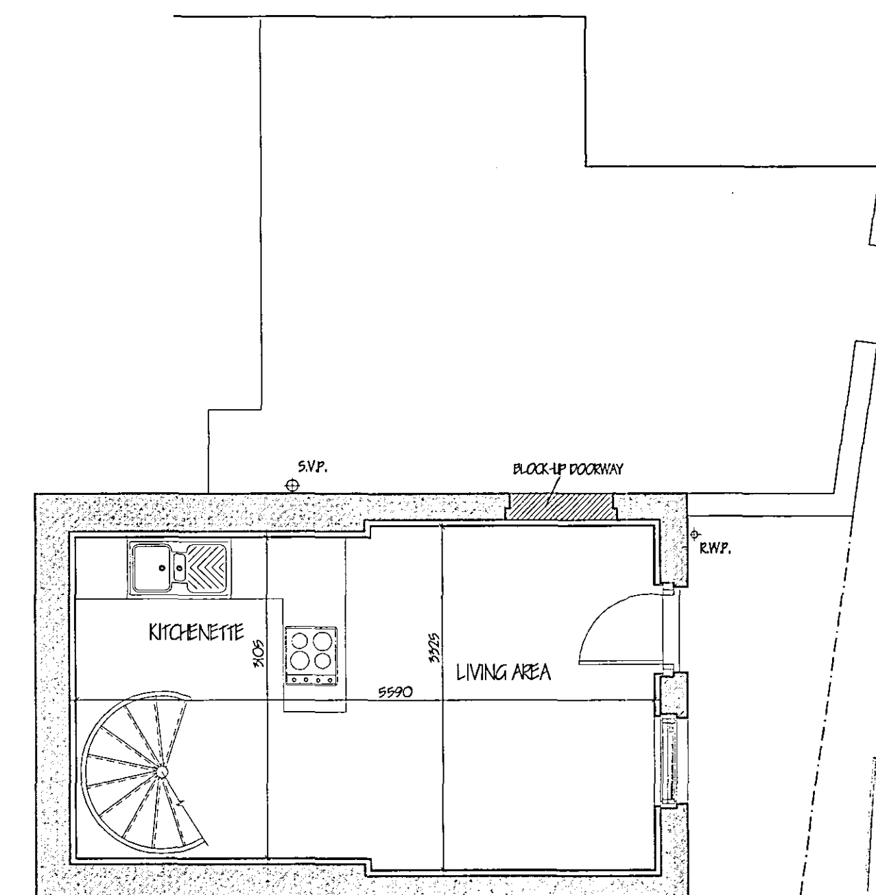
GROUND FLOOR PROPOSED
