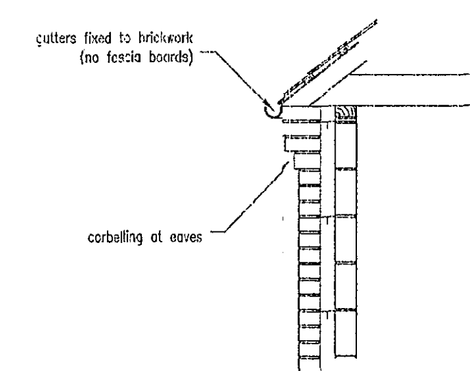
EAVES DETAIL 1:25
