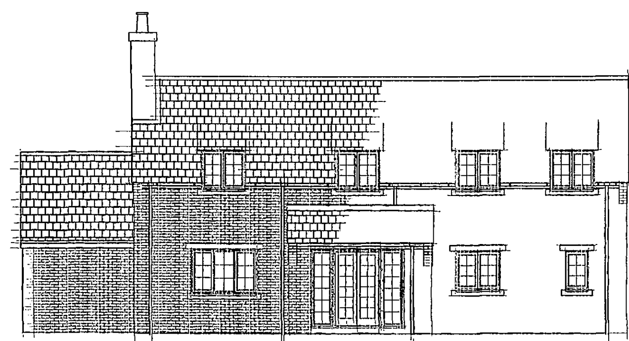
Rear Elevation
