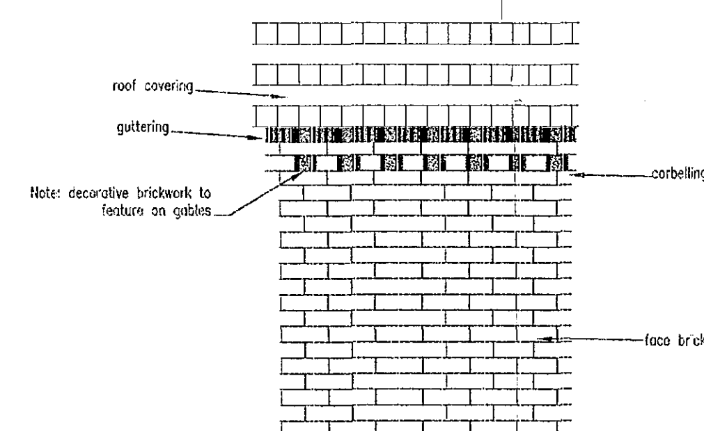
EAVES DETAIL 1:25
