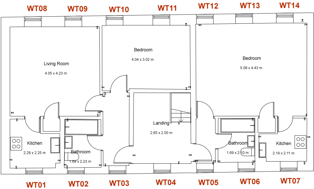
Existing Third Floor Plan (1:100)
