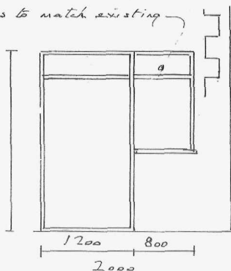
Proposed door and window
