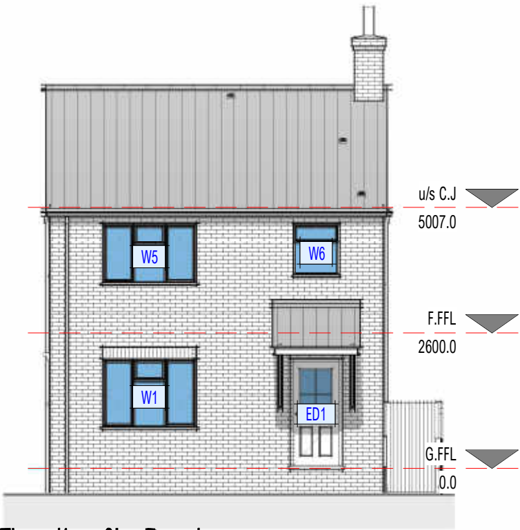
Elevation 01 - Front
