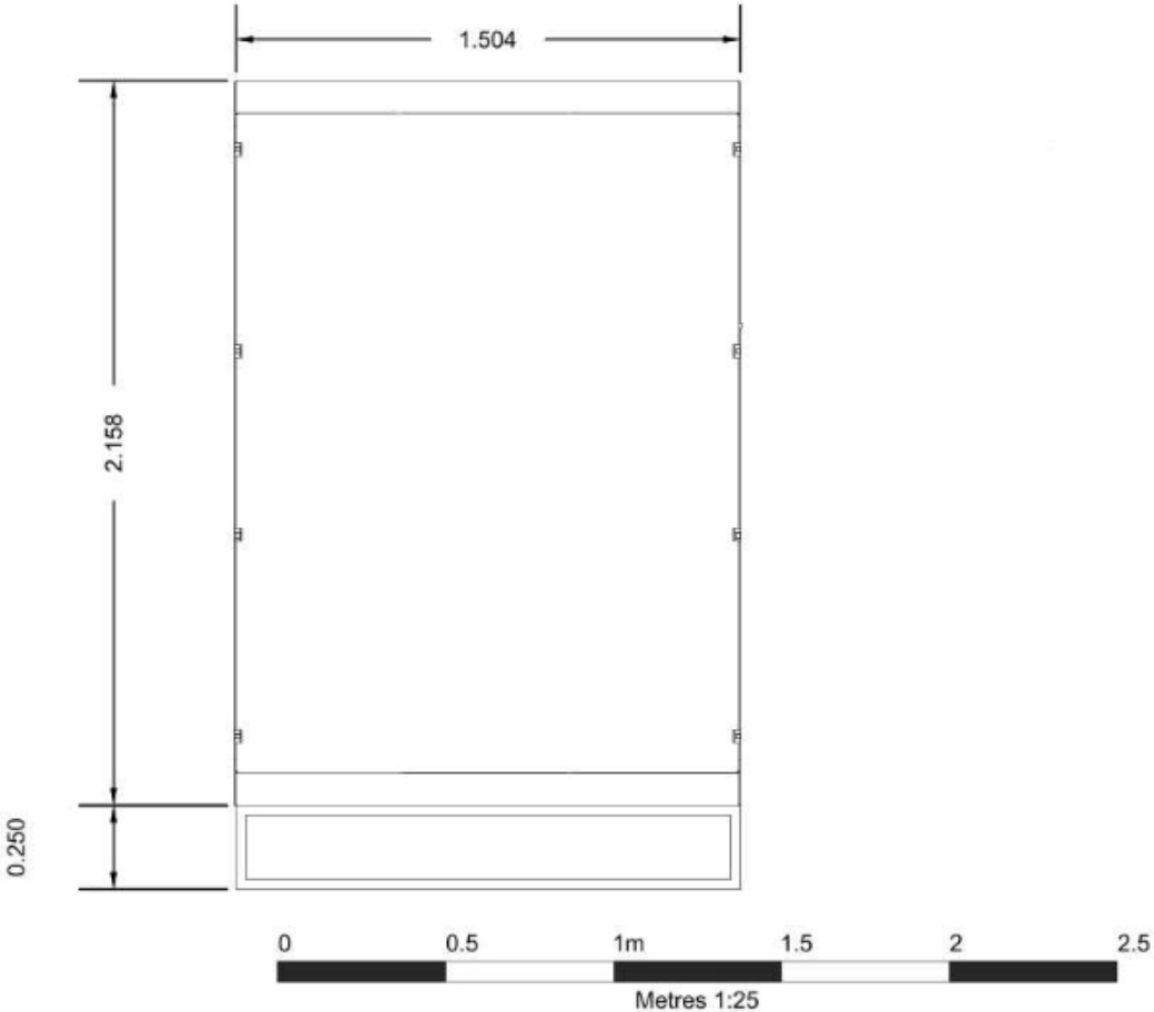
SIDE VIEW
