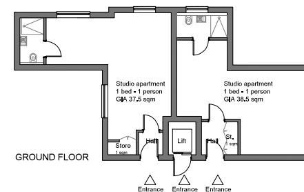
FLOOR PLANS Scale 1:100
