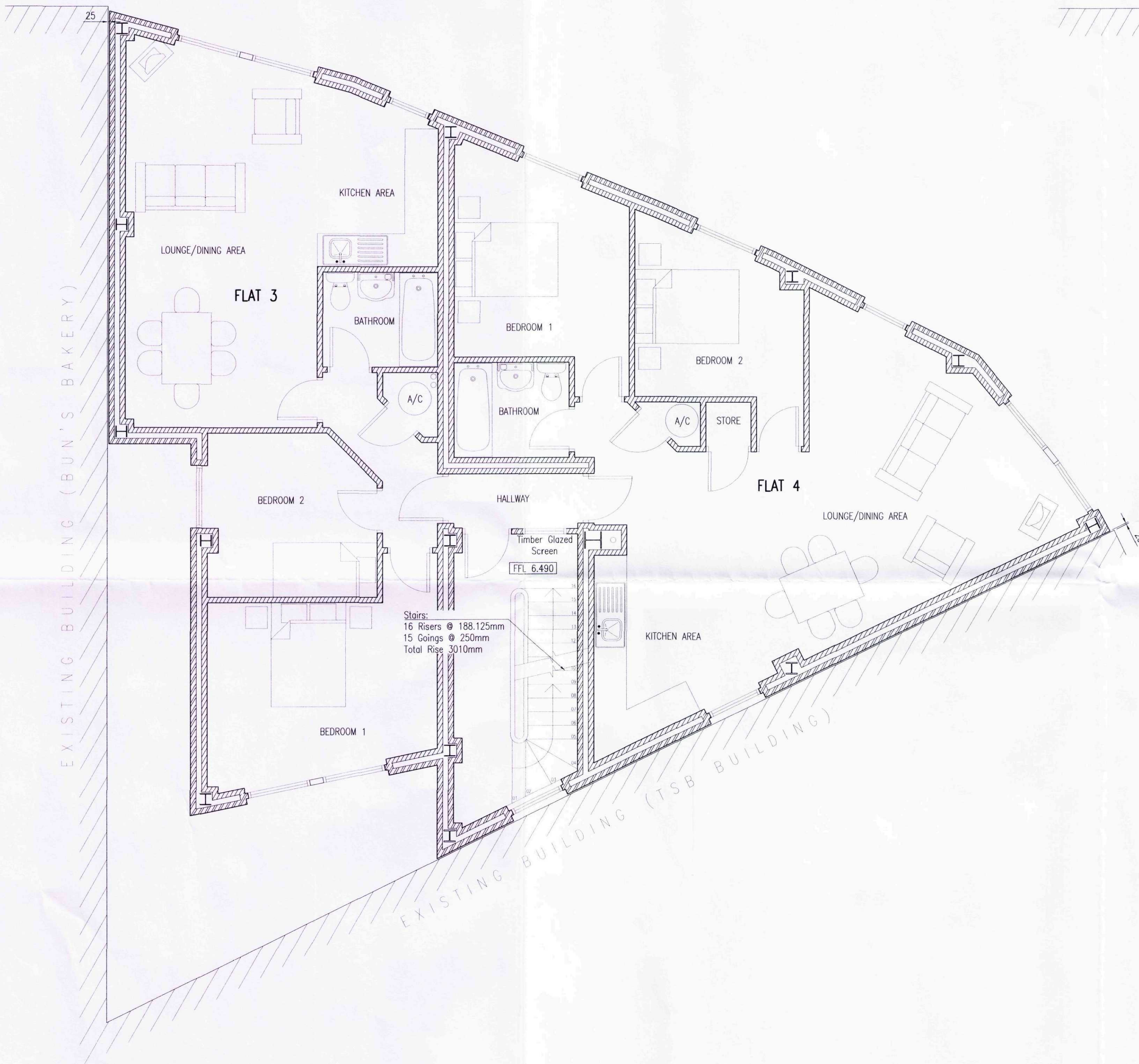
SECOND FLOOR WALL ARRANGEMENT Scale 1:50
