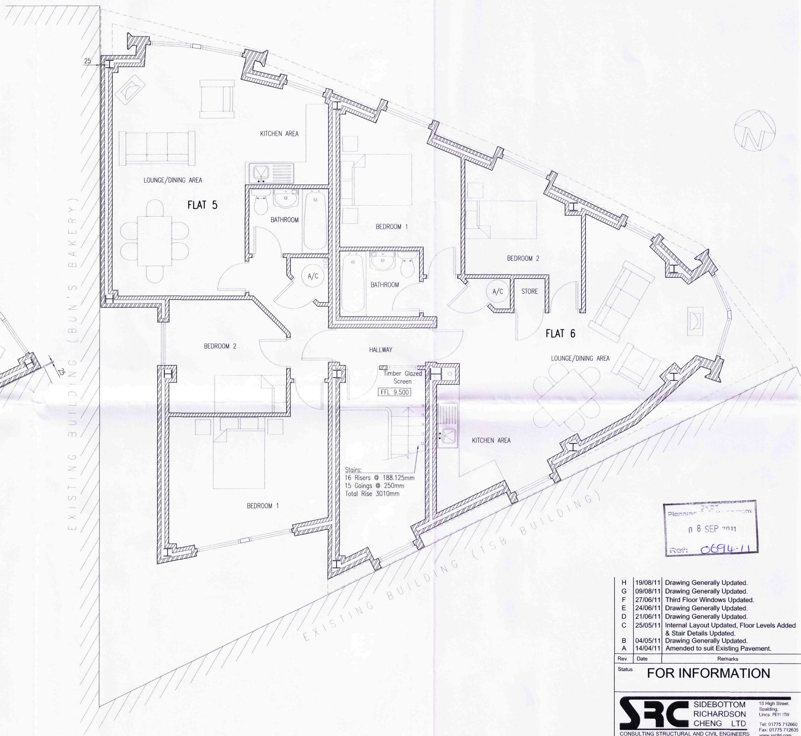
THIRD FLOOR WALL ARRANGEMENT Scale 1:50
