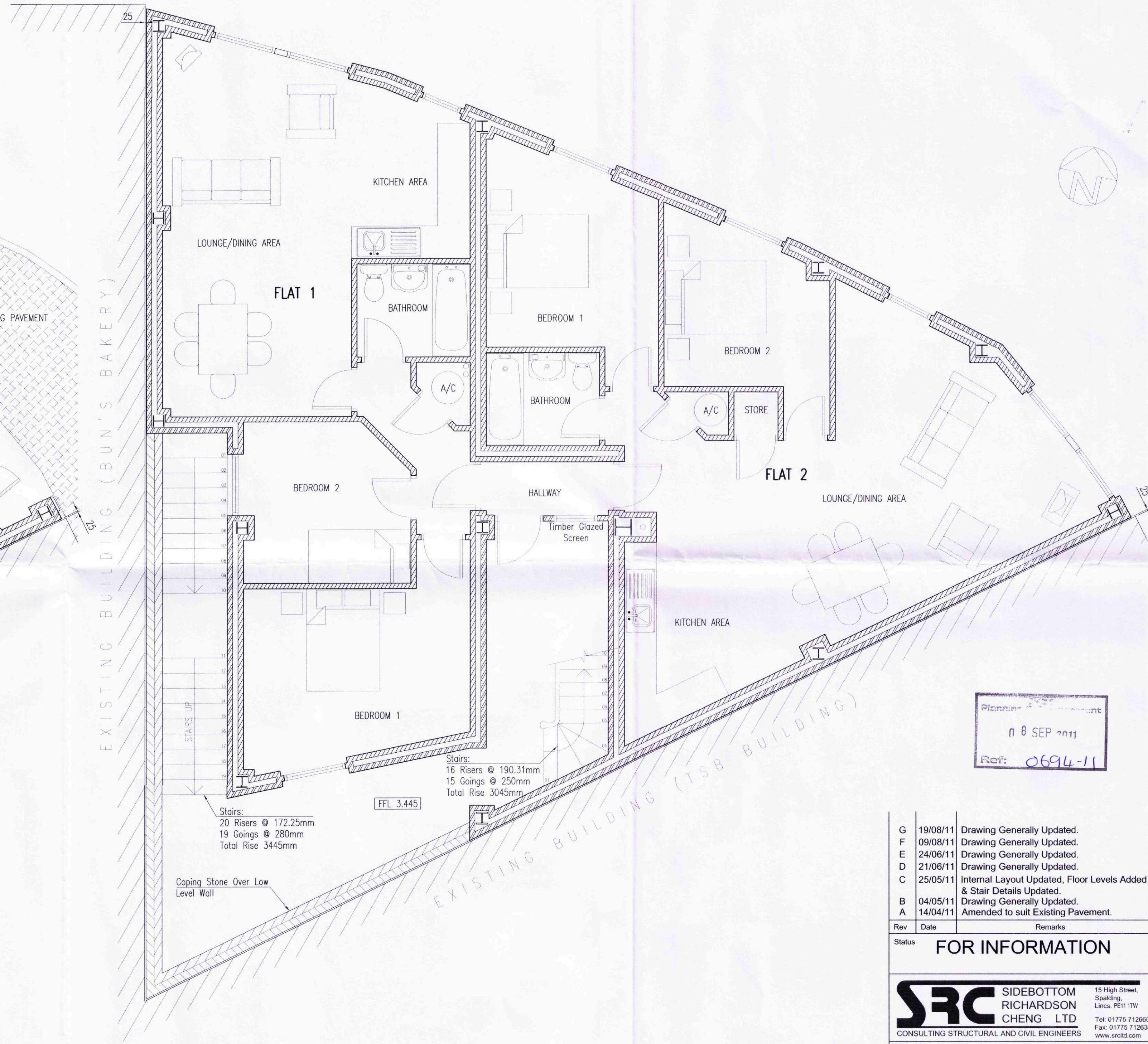
FIRST FLOOR WALL ARRANGEMENT
