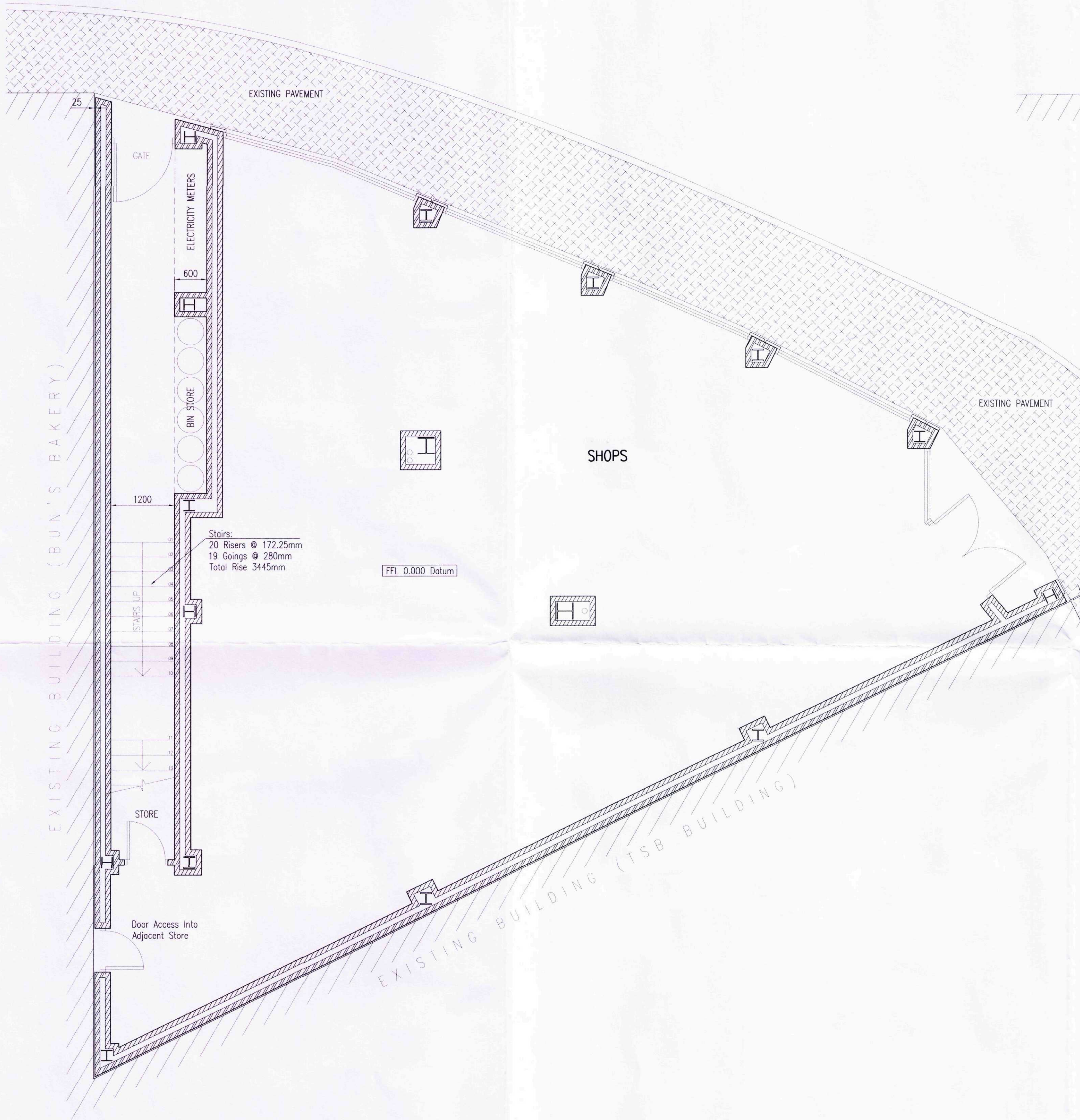
GROUND FLOOR WALL ARRANGEMENT
