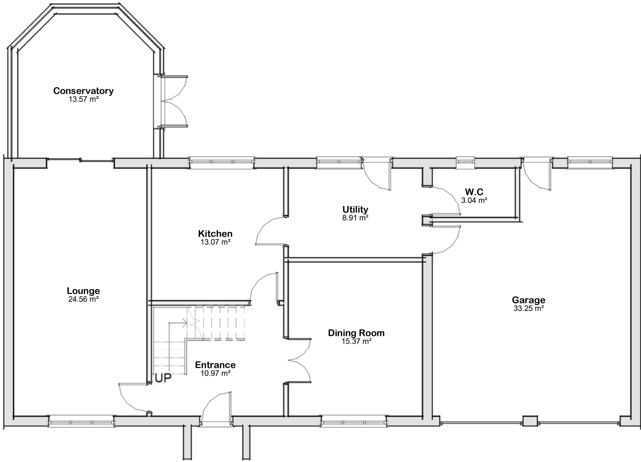
Plan 01 - Ground 1 : 100
