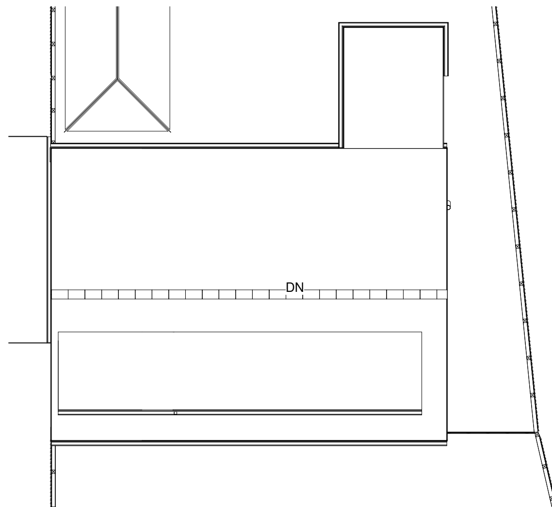
Roof Plan
