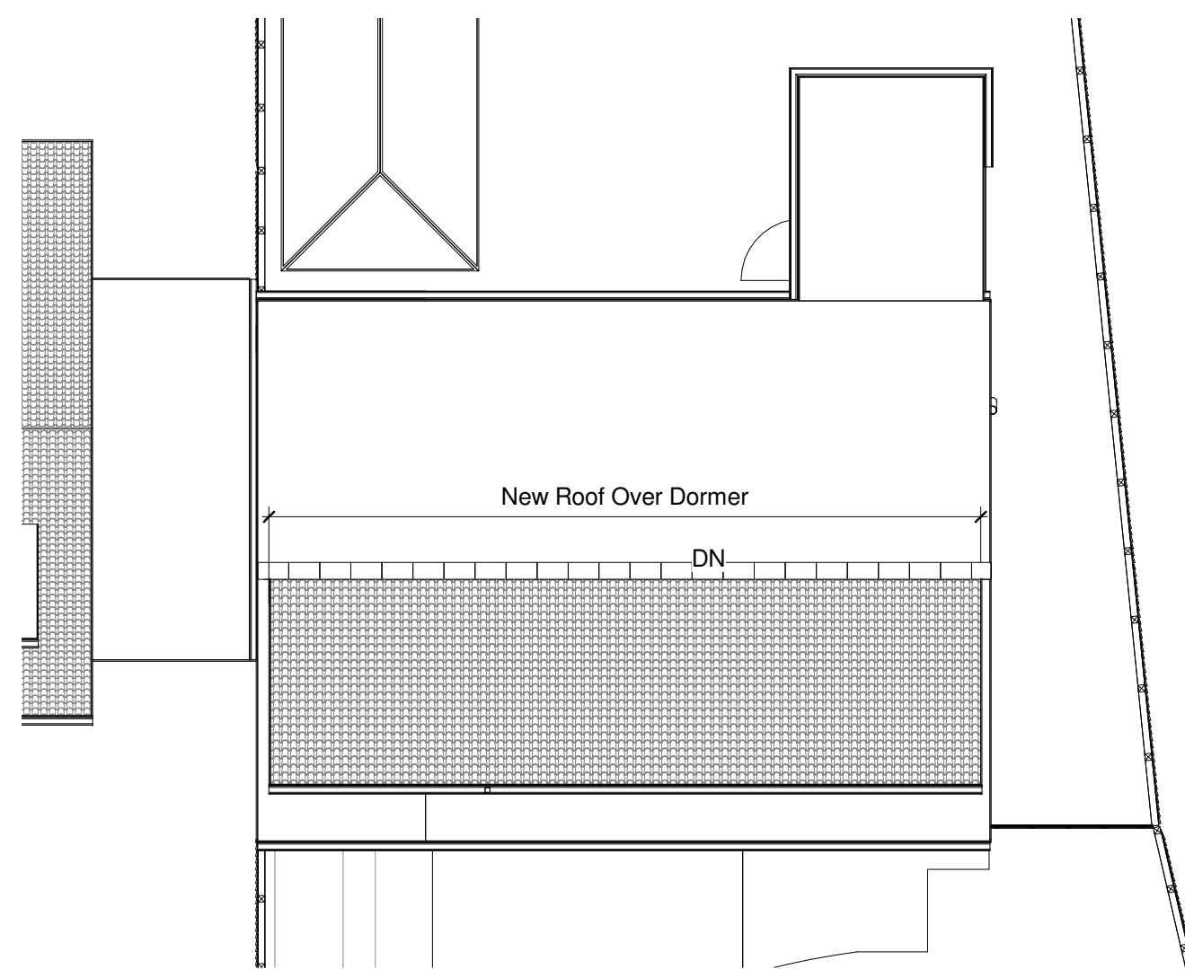
Roof Plan
