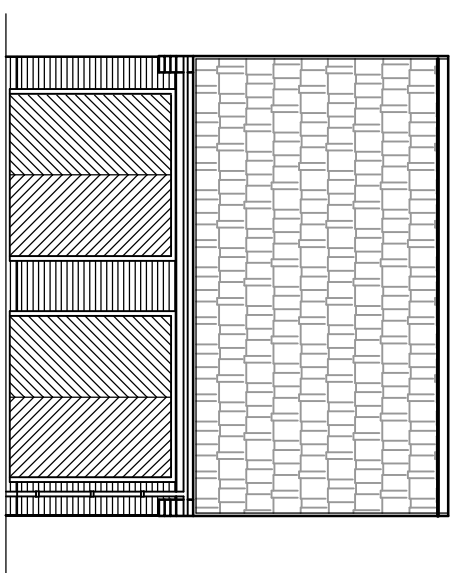
FRONT ELEVATION
