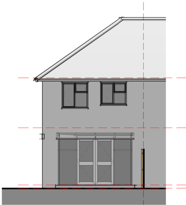
03 - Rear Elevation
