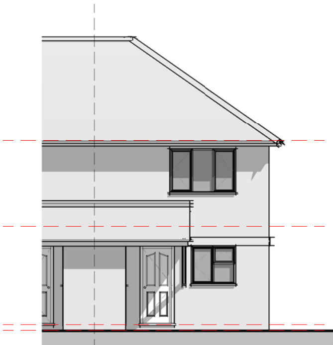
01 - Front Elevation
