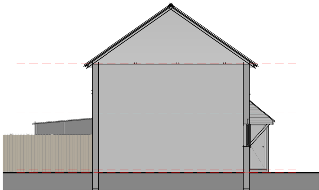
04 - Side Elevation
