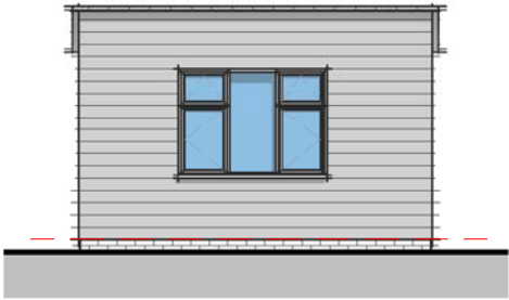
Elevation 01 - Front 1 : 100
