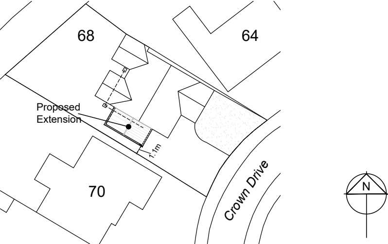
Block Plan - 1:500 scale
