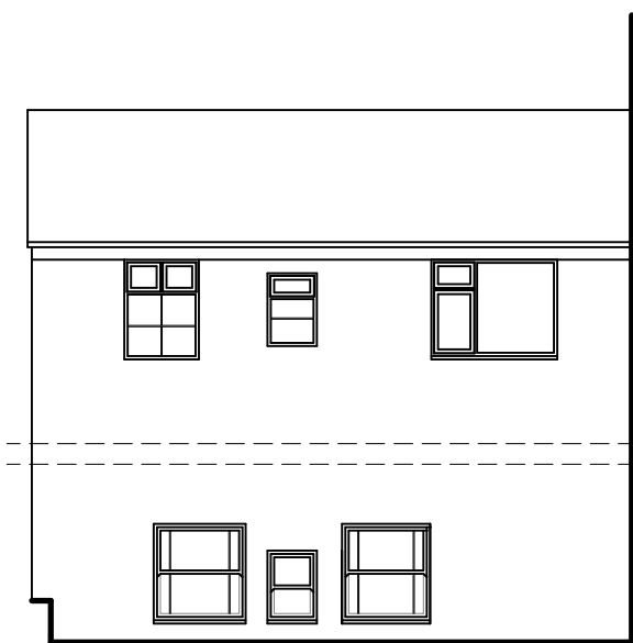
EAST ELEVATION
