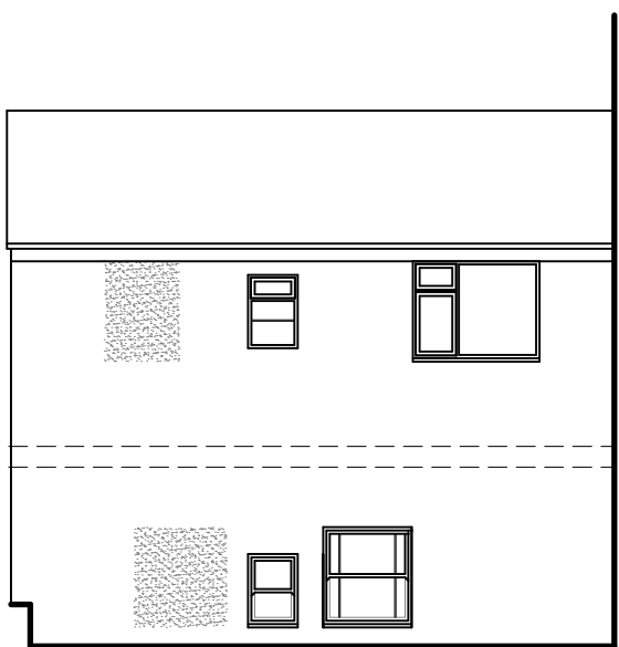
EAST ELEVATION
