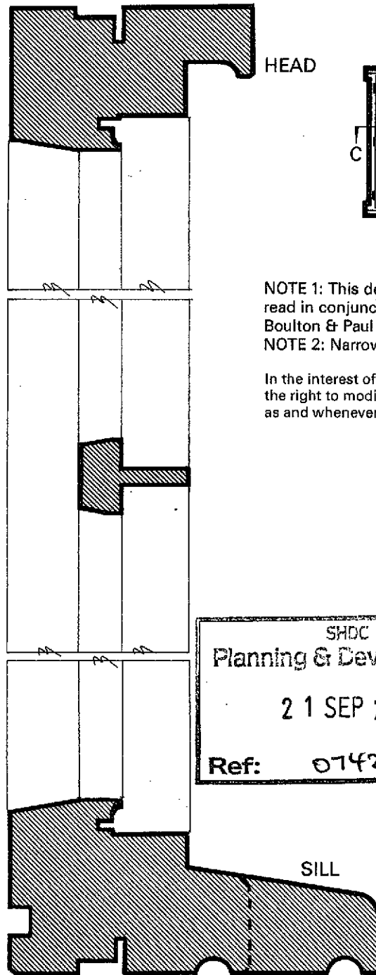
Section BB
