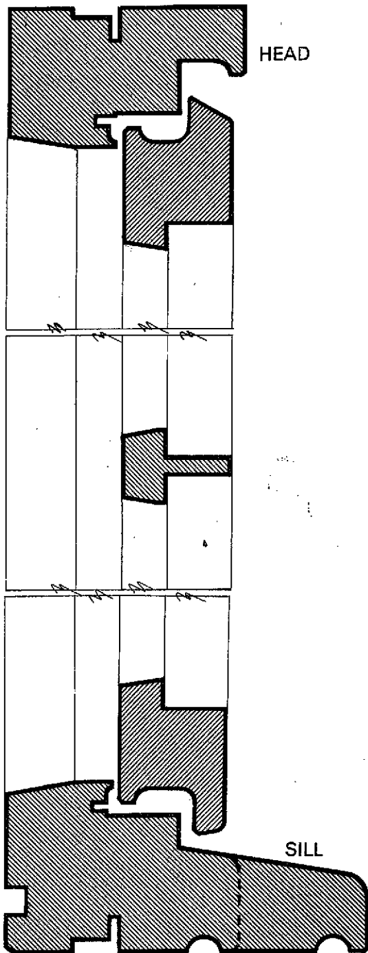
Section AA
