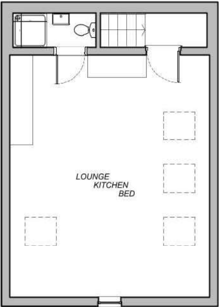
PROPOSED FF PLAN SCALE 1:100
