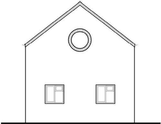
PROPOSED FRONT ELEVATION SCALE 1:100
