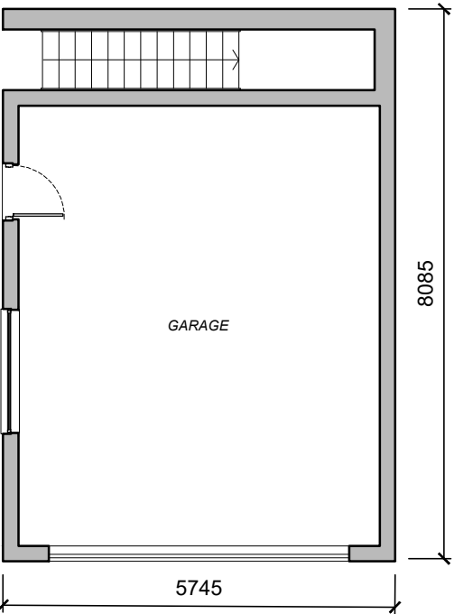
EXISTING GF PLAN SCALE 1:100
