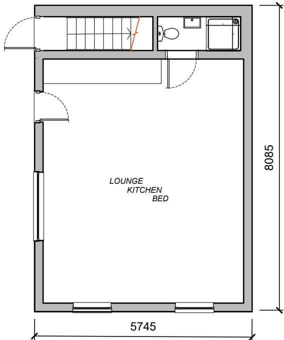
PROPOSED GF PLAN SCALE 1:100
