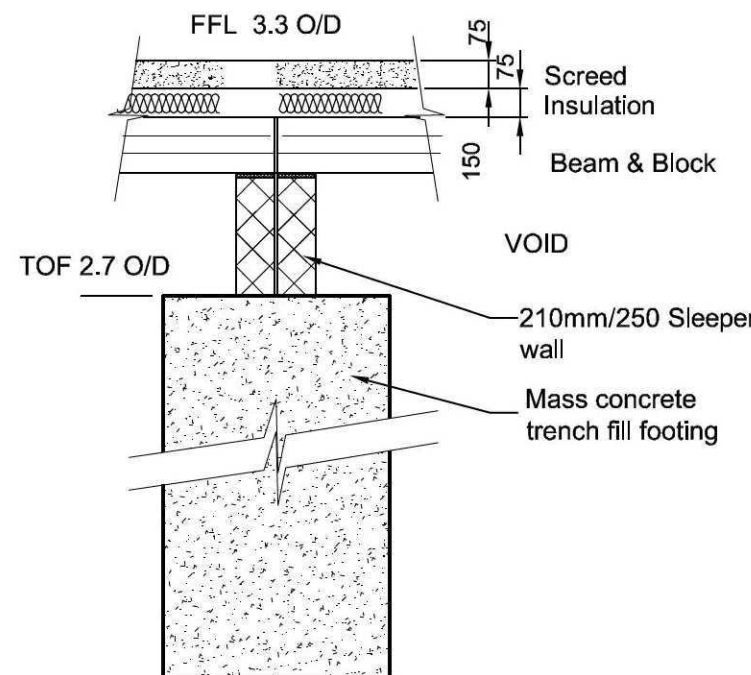
SECTION C-C SCALE 1:20
