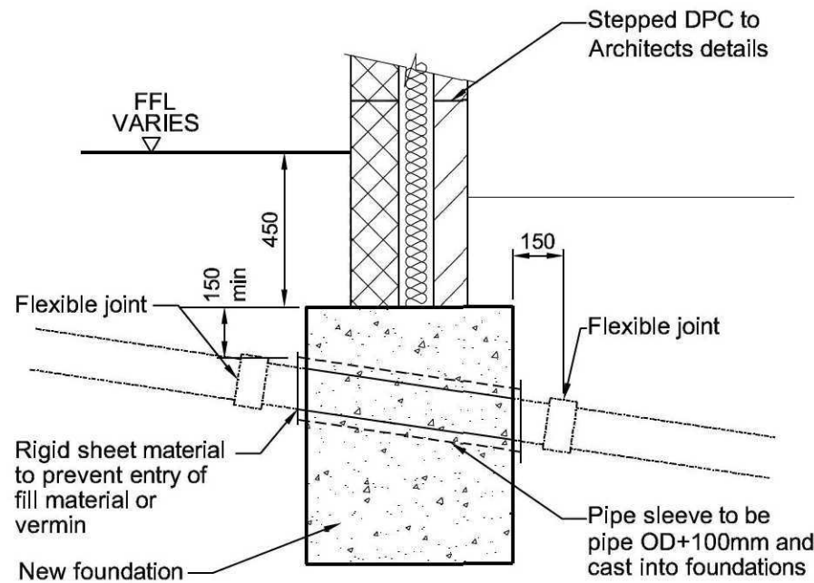
TYPICAL DRAINAGE DETAIL THROUGH FOUNDATION SCALE 1:20
