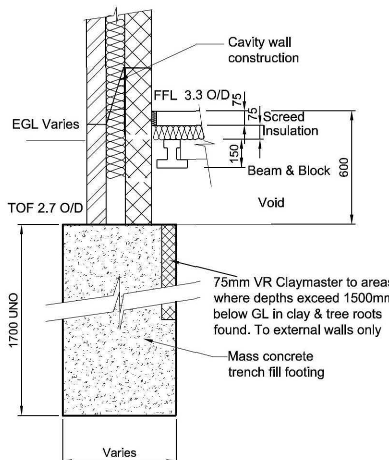
TYPICAL EDGE DETAIL (SECTION A-A) SCALE 1:20
