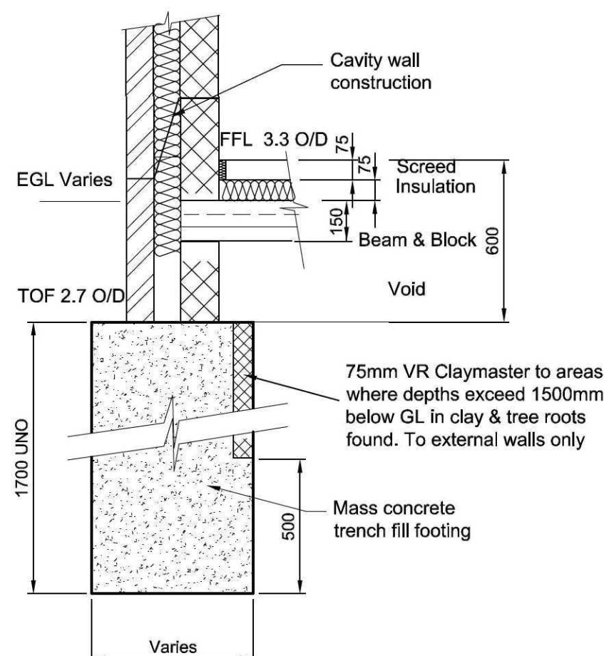
TYPICAL EDGE DETAIL (SECTION B-B) SCALE 1:20
