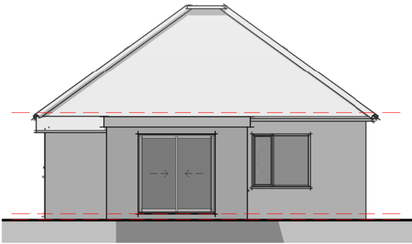
Elevation 03 - Rear 1 : 100
