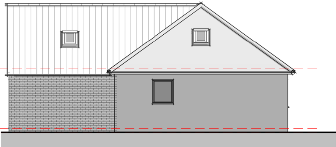
Elevation 04 – Left 1 : 100
