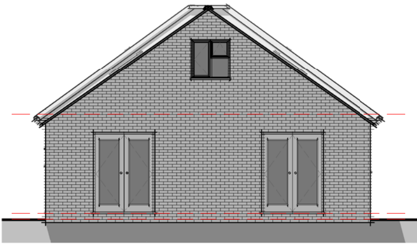
Elevation 03 – Rear 1 : 100
