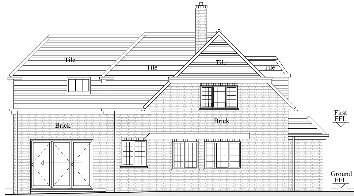
Proposed Side 2 Elevation
