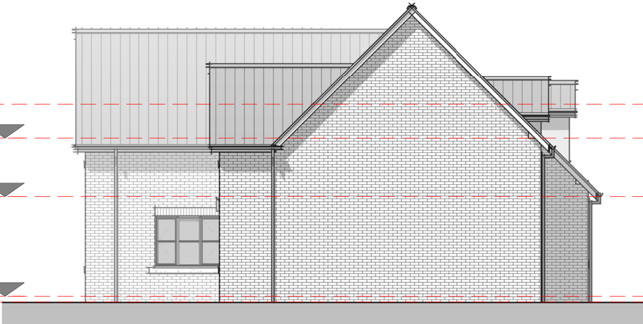
Elevation 02 – Right 1 : 100
