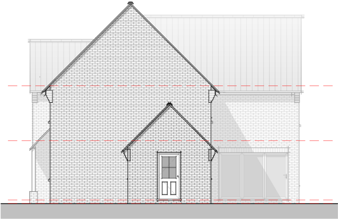
Elevation 02 – Right 1 : 100
