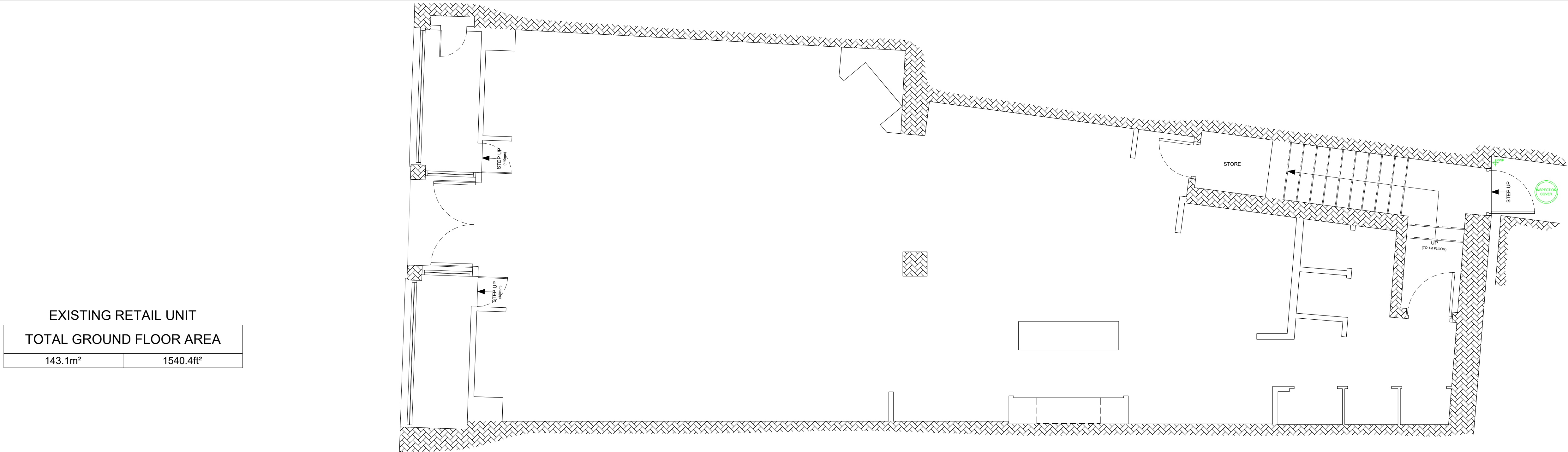
EXISTING GROUND FLOOR GENERAL ARRANGEMENT PLAN
