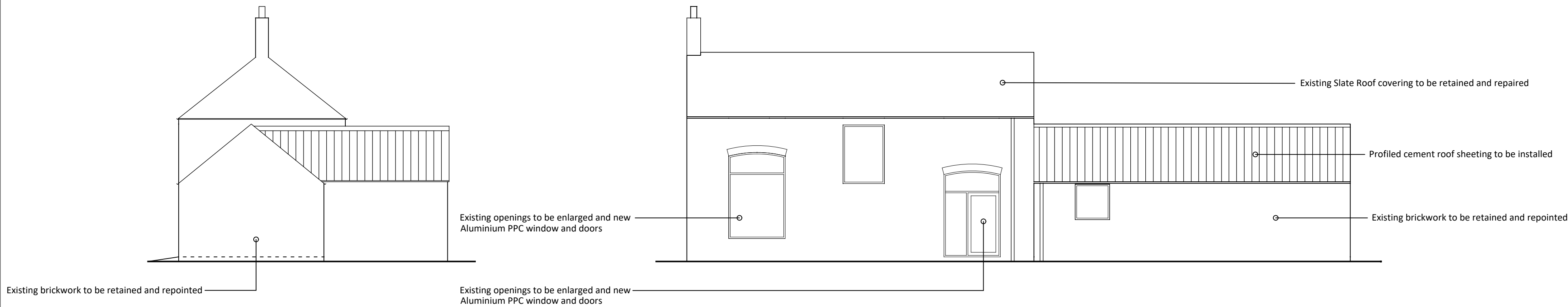
Proposed West Elevation
