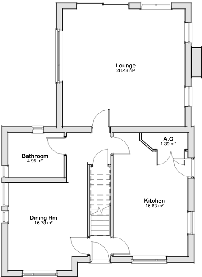
01 - Ground Floor Plan 1 : 100
