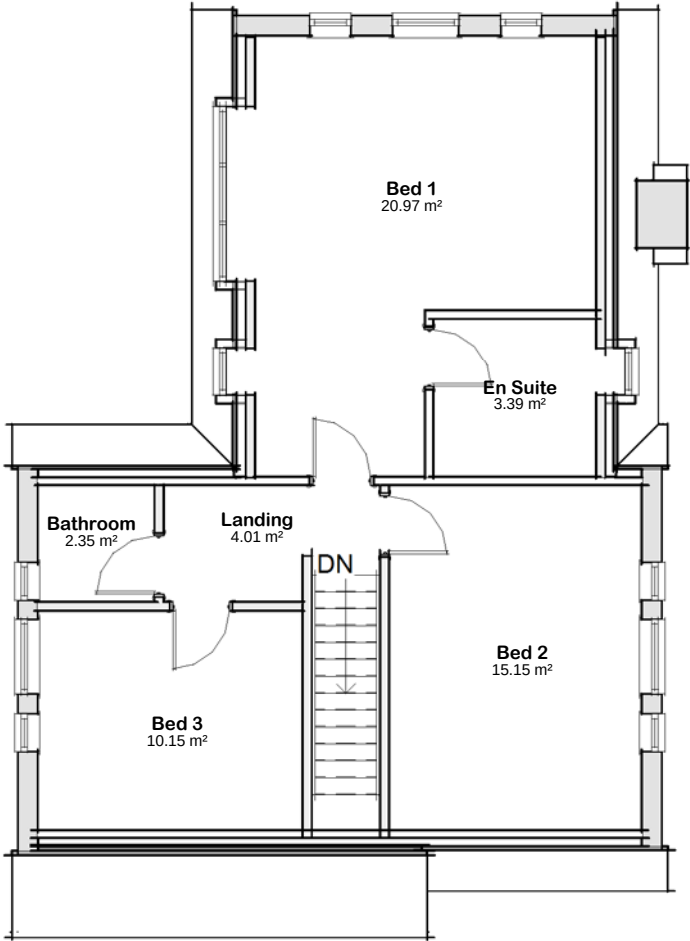
02 - 1st Floor Plan 1 : 100
