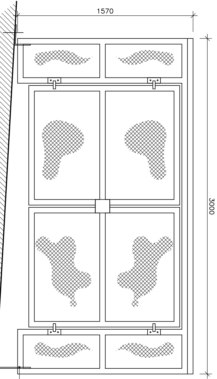
FRONT ELEVATION
