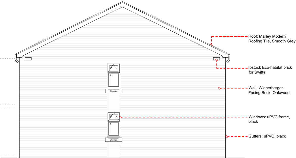
NORTH ELEVATION @ 1:100
