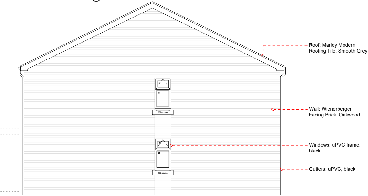
REAR ELEVATION @ 1:100
