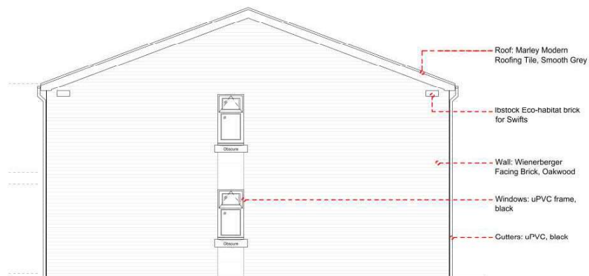
NORTH ELEVATION @ 1:100
