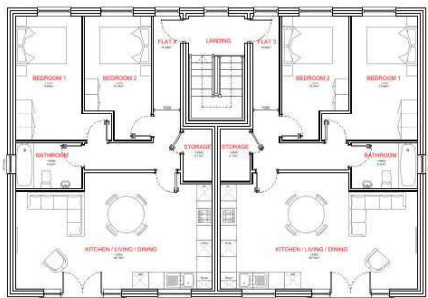
FIRST FLOOR PLAN @ 1:200
