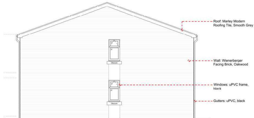
SOUTH ELEVATION @ 1:100
