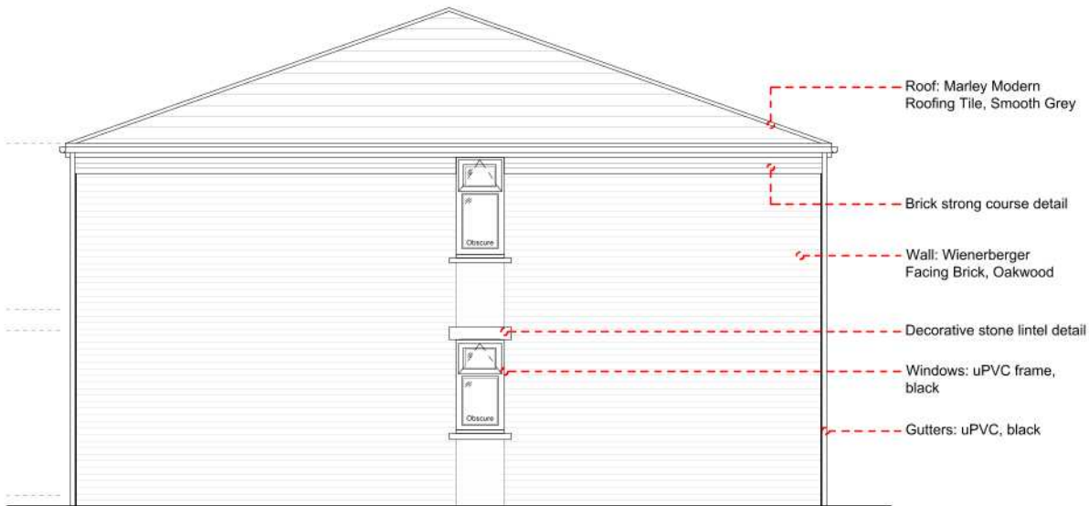
SOUTH ELEVATION @ 1:100
