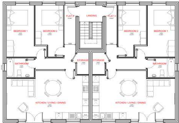
FIRST FLOOR PLAN @ 1:200
