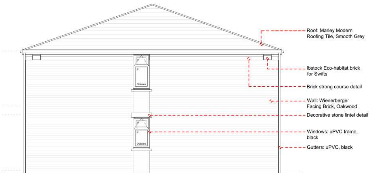
NORTH ELEVATION @ 1:100
