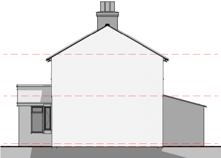
Elevation 02 – Right 1 : 100
