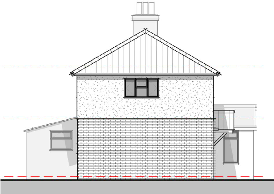
Elevation 04 – Left 1 : 100
