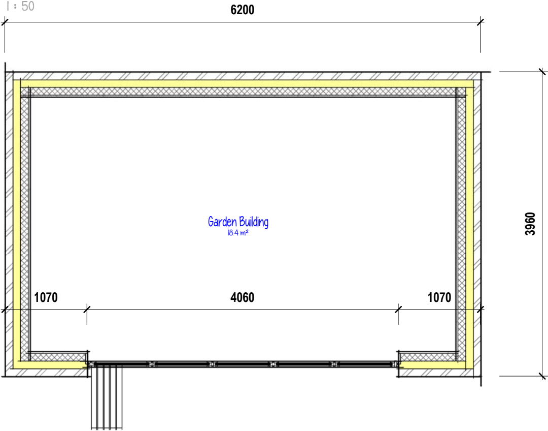
Plan 01 - Ground I : 50
