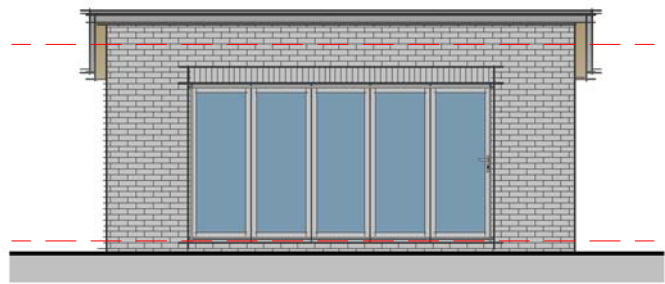
Elevation 01 - Front I : 100
