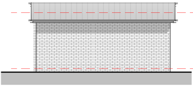
Elevation 03 - Rear I : 100
