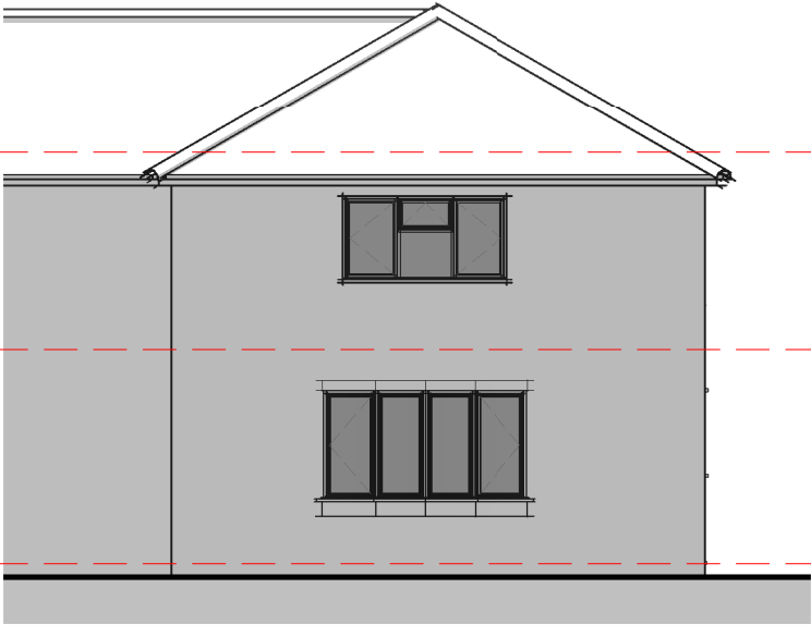
Elevation 01 - Front 1 : 100
