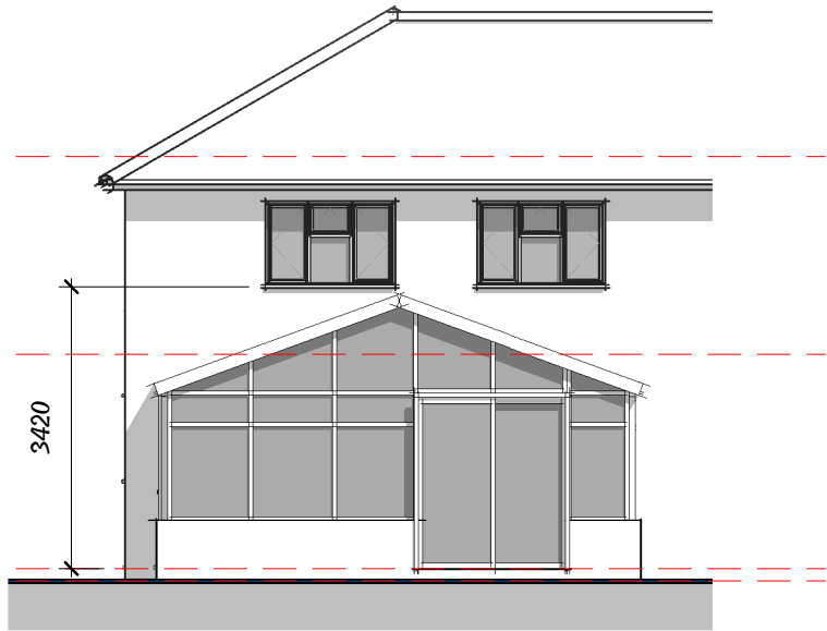
Elevation 03 - Rear 1 : 100
