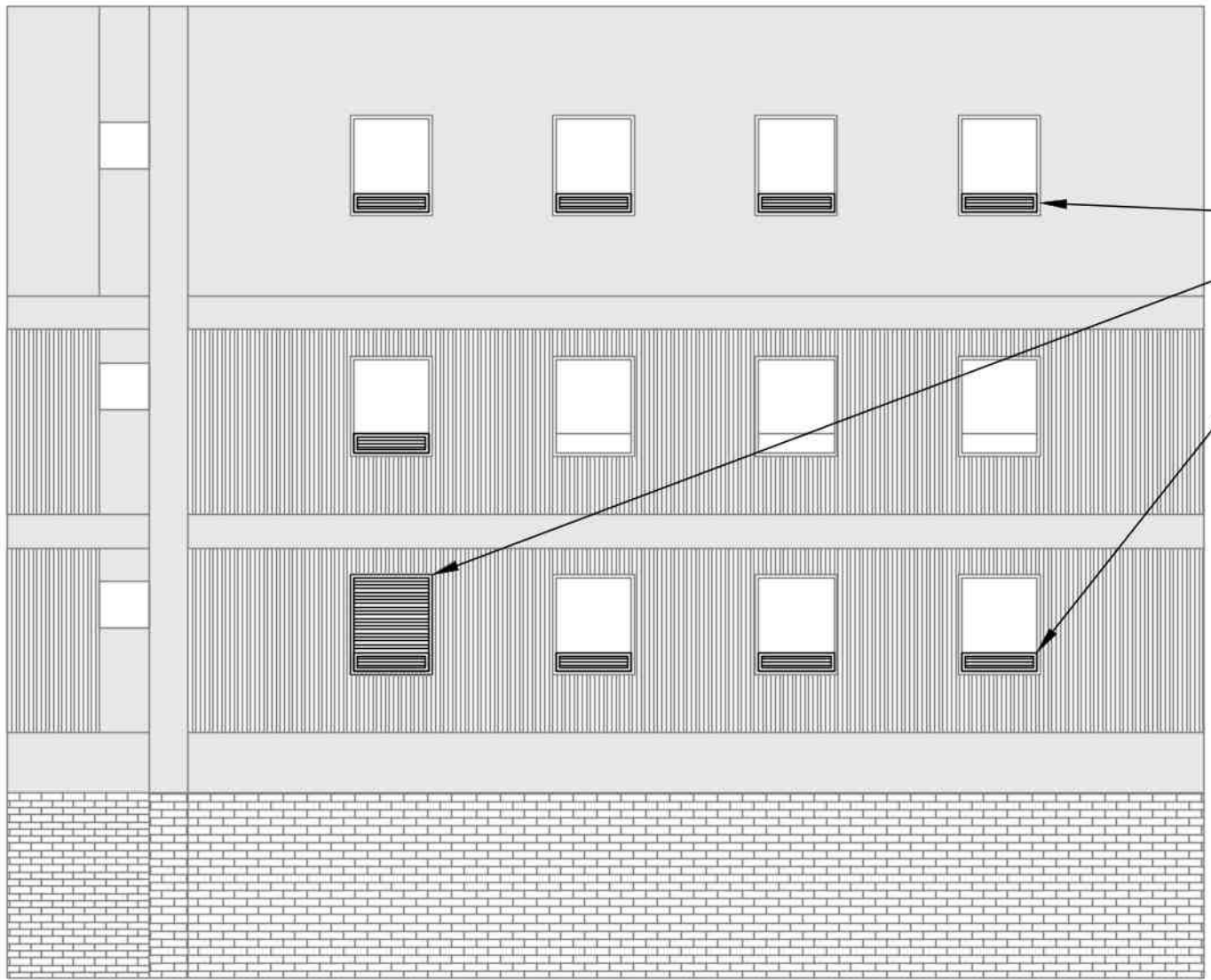
EXISTING SOUTH ELEVATION (1:100)
