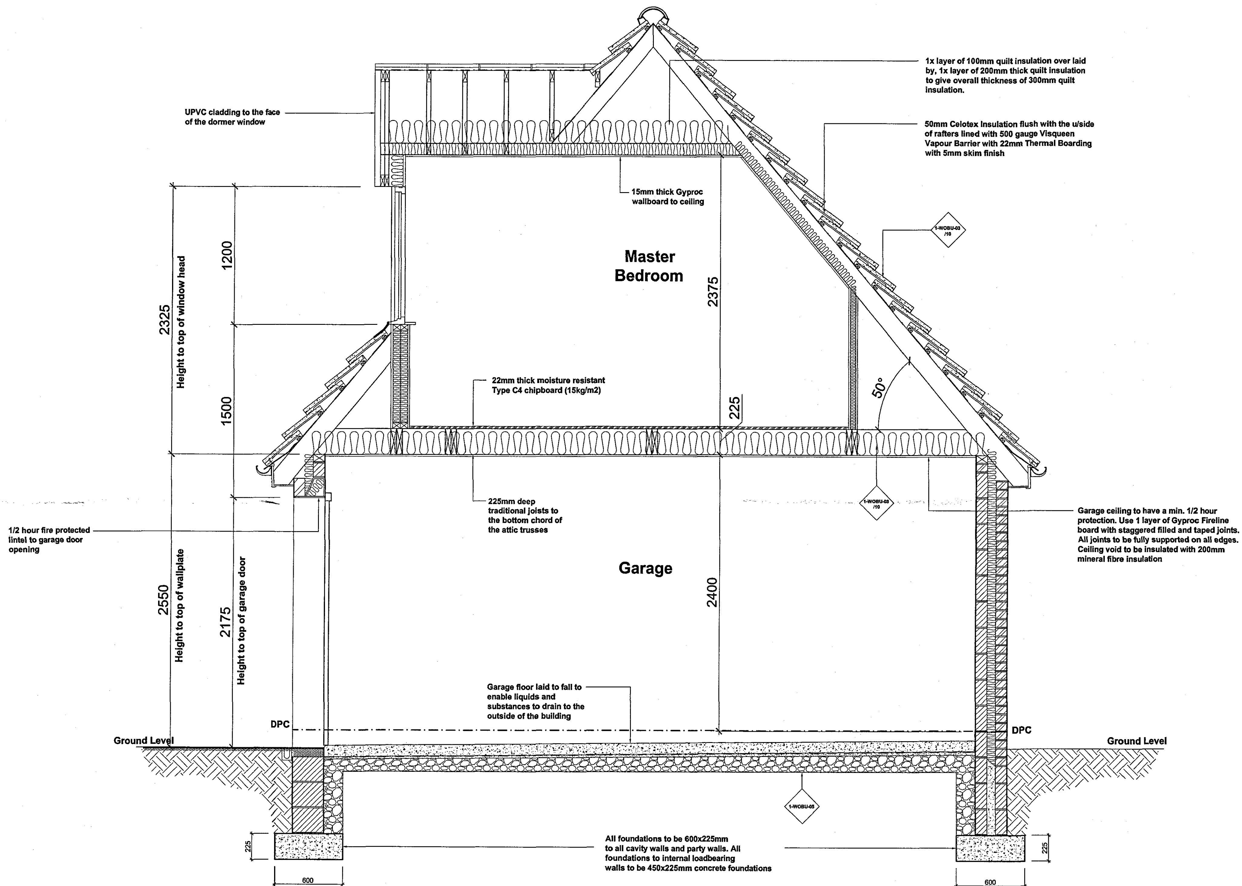
Section B-B
