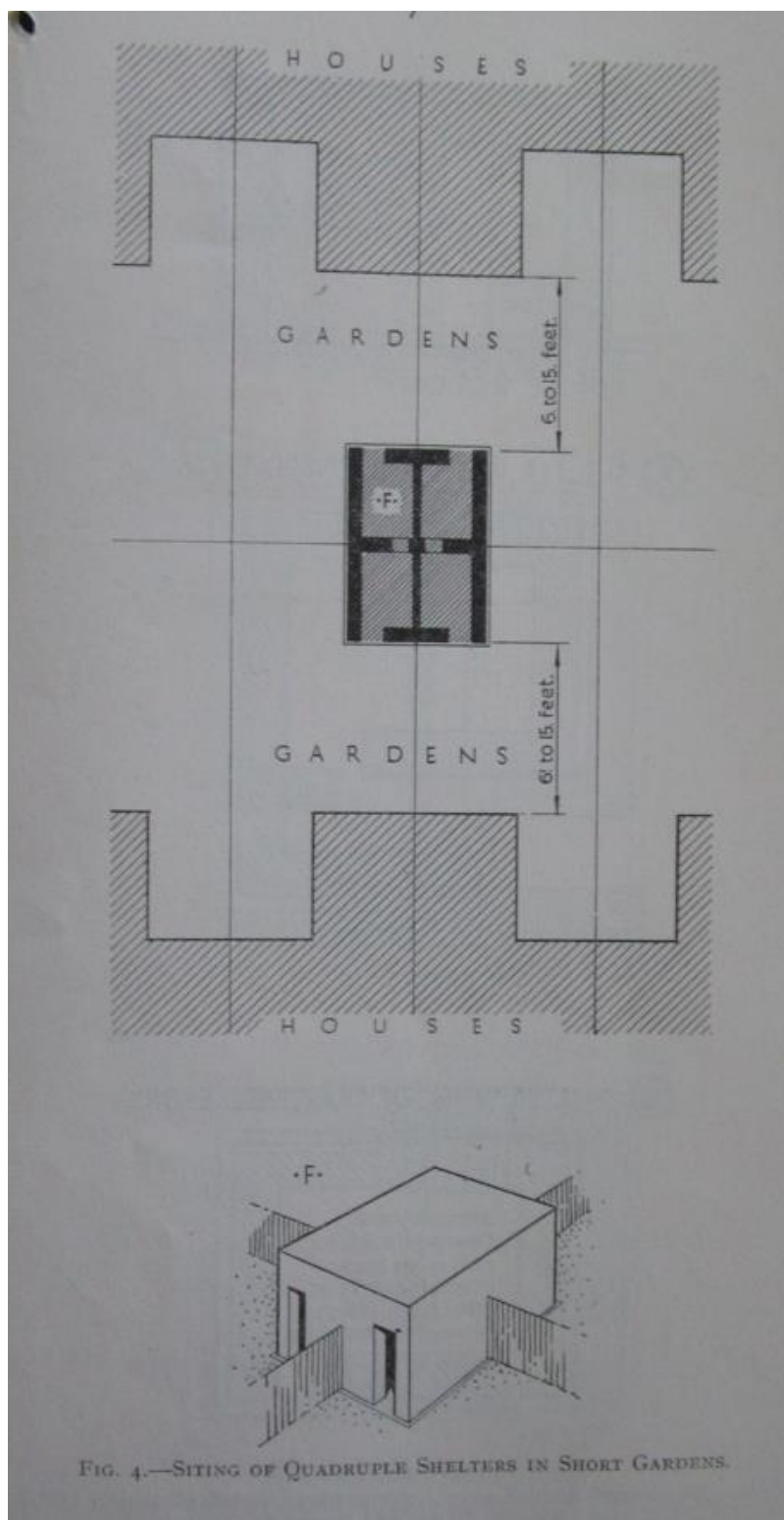
Historical Plate 14: Siting of quadruple domestic surface shelter in gardens, from Directions for the Erection of Domestic Surface Shelters , May 1939 © The National Archives HO 205/153
