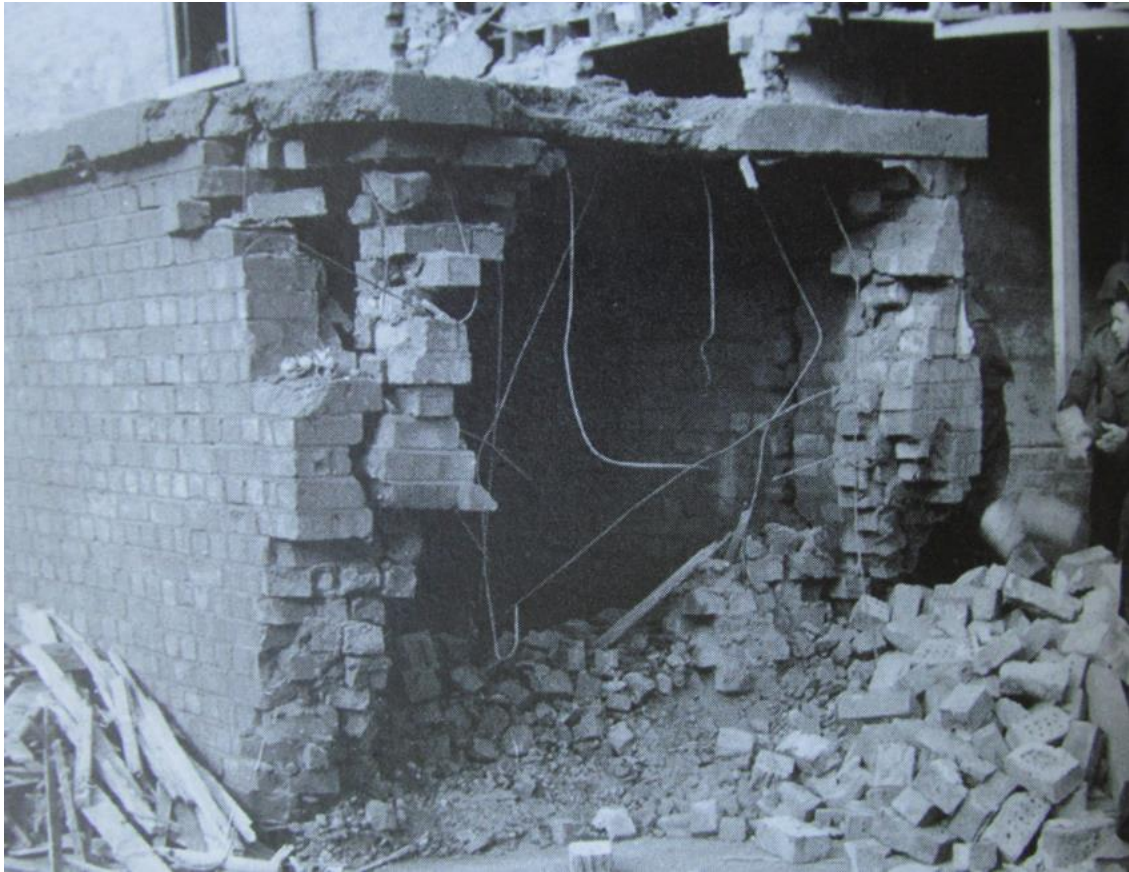
Historical Plate 17: Bomb damaged brick and concrete surface shelter at Bellamy's house and stables, Lincoln, showing reinforcing bars in the brickwork, in accordance with Circular 290/40 (Source: Wade 2011: 48)
