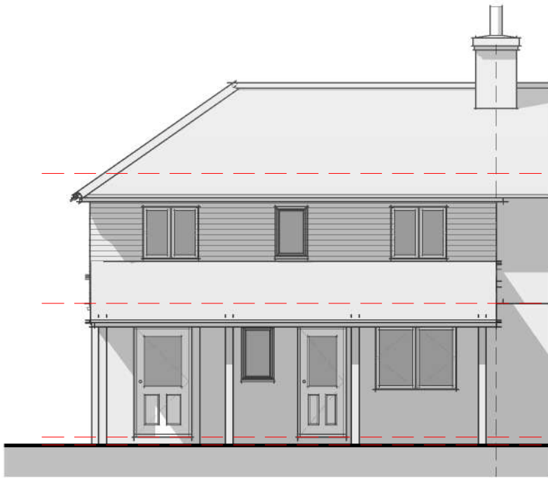
Elevation 03 - Rear 1 : 100
