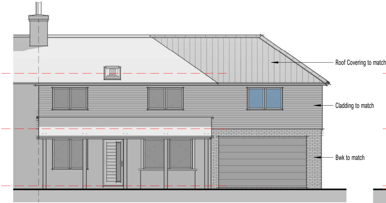
Elevation 01 - Front 1 : 100
