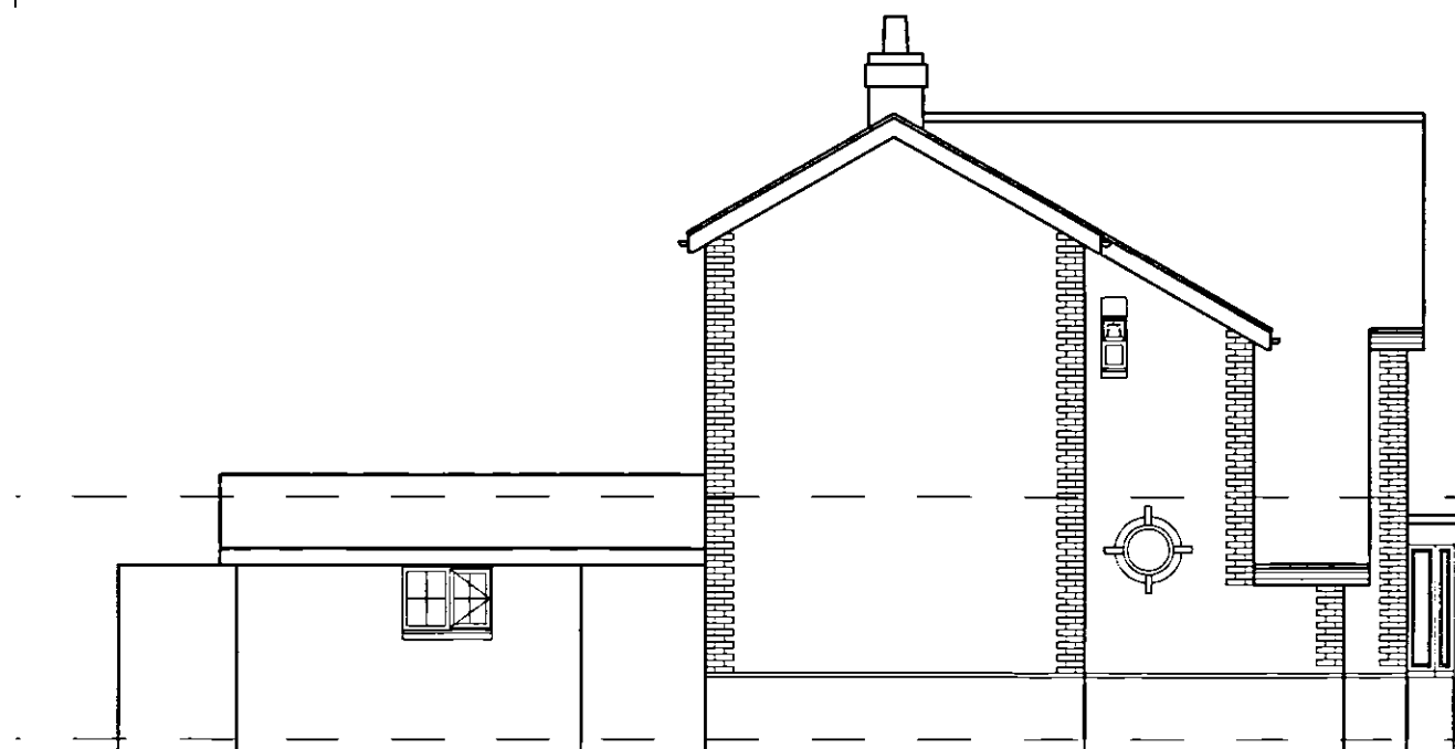
South Elevation
