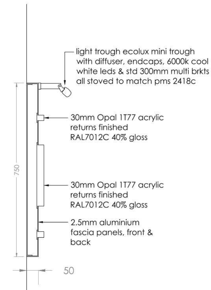
SECTION THROUGH FASCIA 1:10@A3
