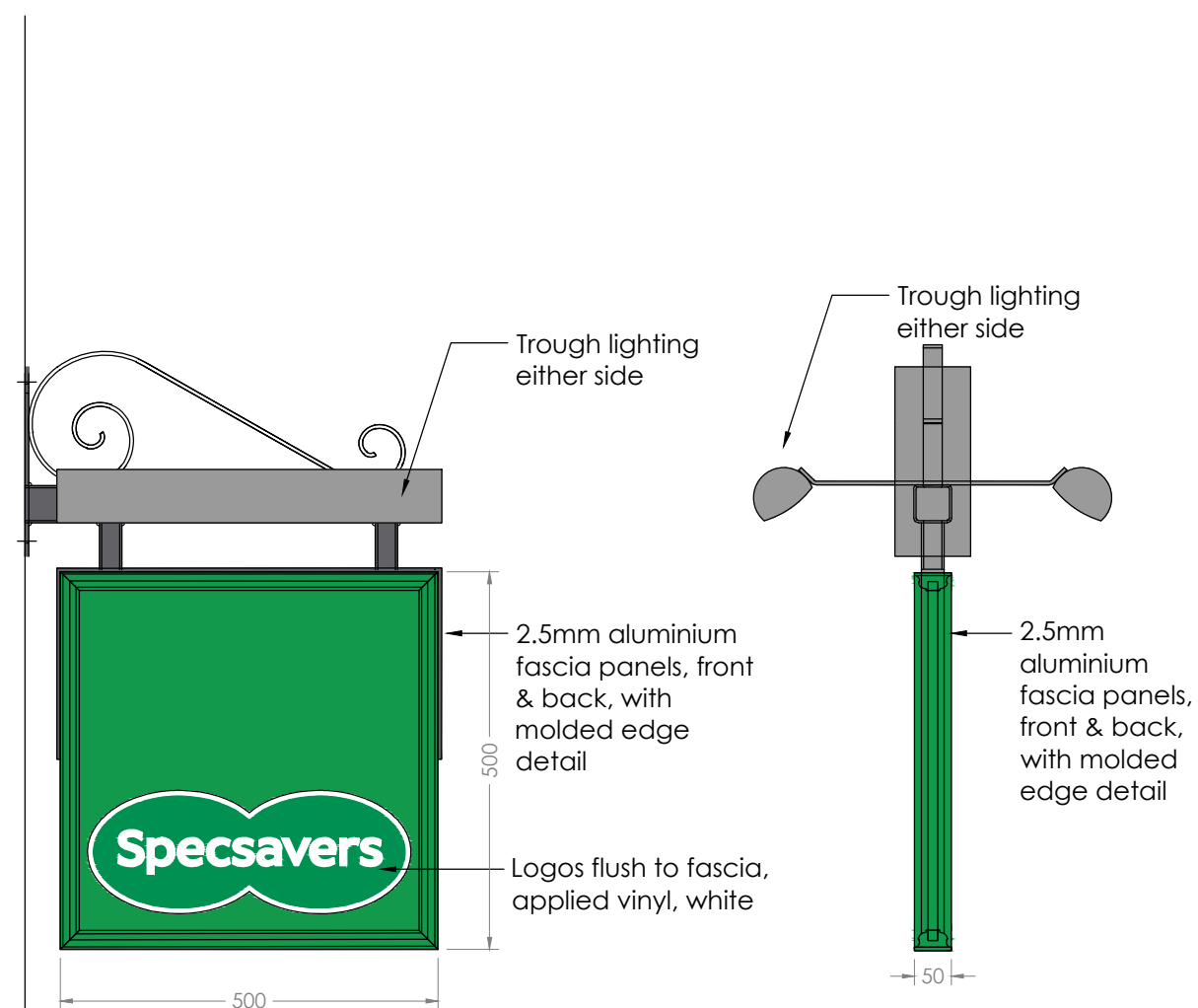
PROJECTING SIGN - EXTERNAL ILLUMINATION 1:10@A3
