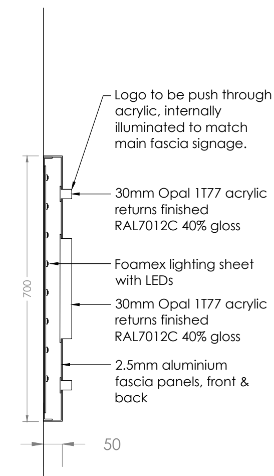
SECTION THROUGH FASCIA 1:10@A3
