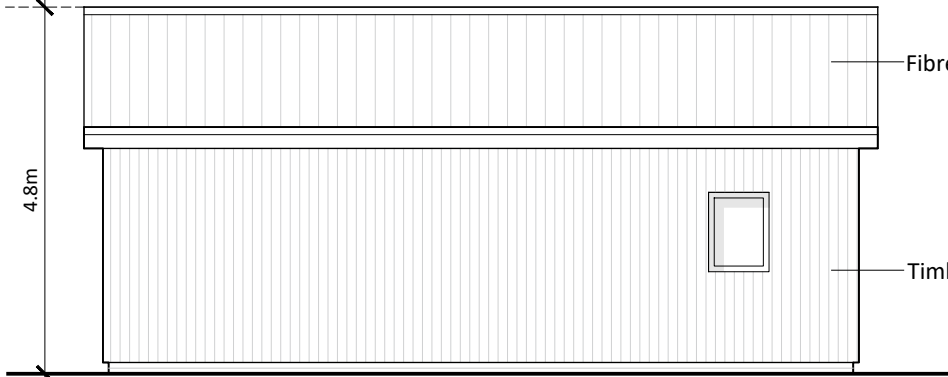
West Elevation
