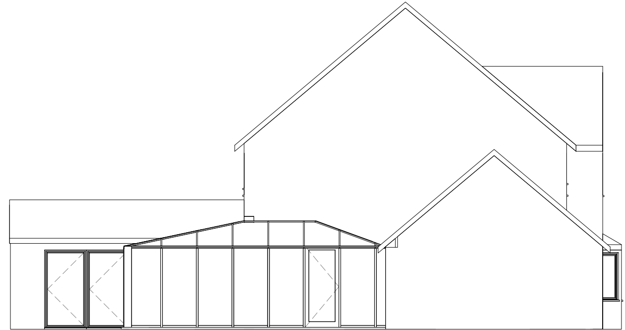
2 NE Elevation - (Existing) 1 : 100
