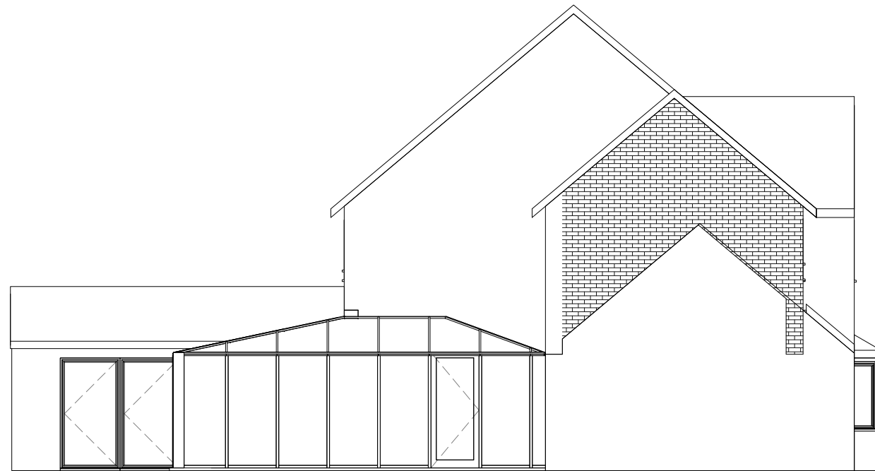
2 NE Elevation - (Proposed) 1 : 100
