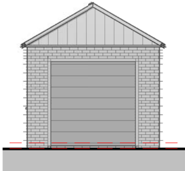
Elevation 03 - Rear 1 : 100
