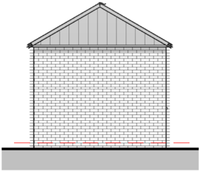
Elevation 01 - Front 1 : 100
