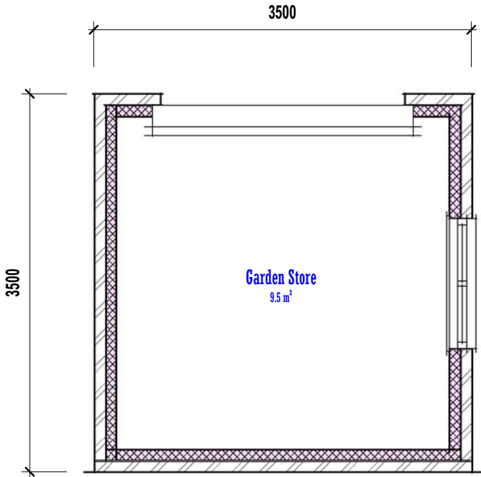
Plan 01 - Ground 1 : 50
