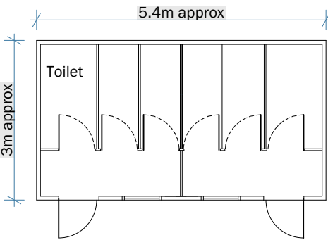
Plans
