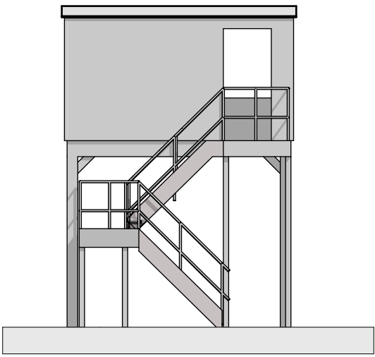
West Facing Elevation
