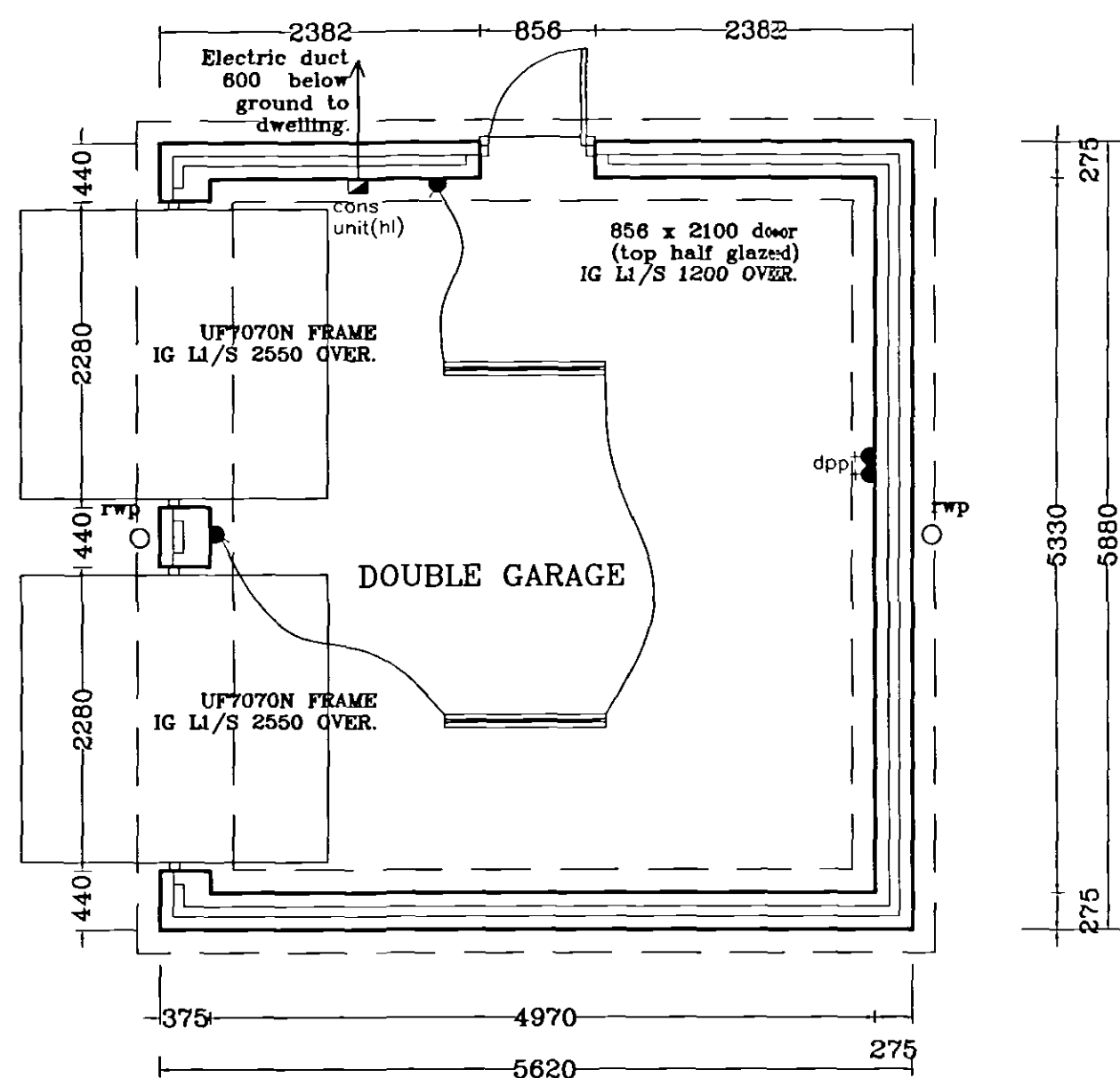
FLOOR LAYOUT
